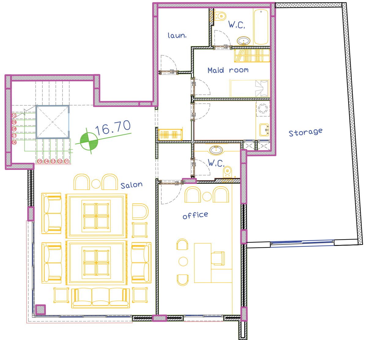
Villa 27 Basement Plan
